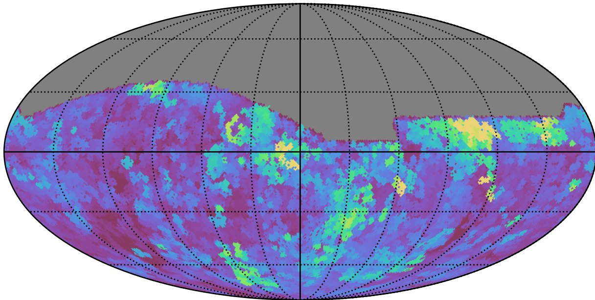
too_elab_r16_d3_giz_v3.4_10yrs All sky g band: Max seeingEff
