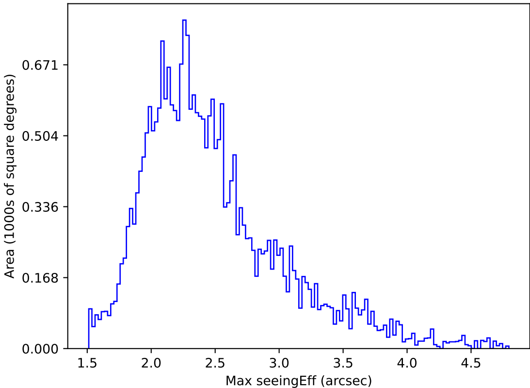
too_elab_r16_d3_giz_v3.4_10yrs All sky g band: Max seeingEff
