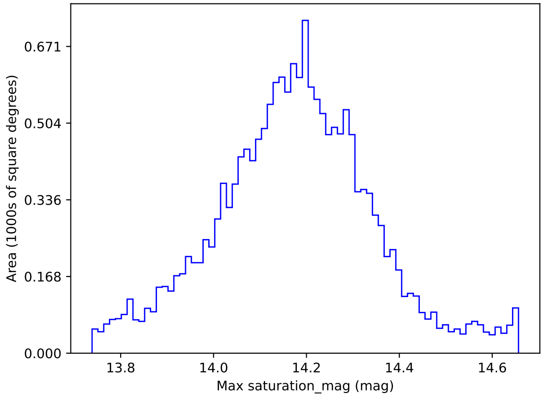
too_elab_r16_d3_giz_v3.4_10yrs WFD y band: Max saturation_mag
