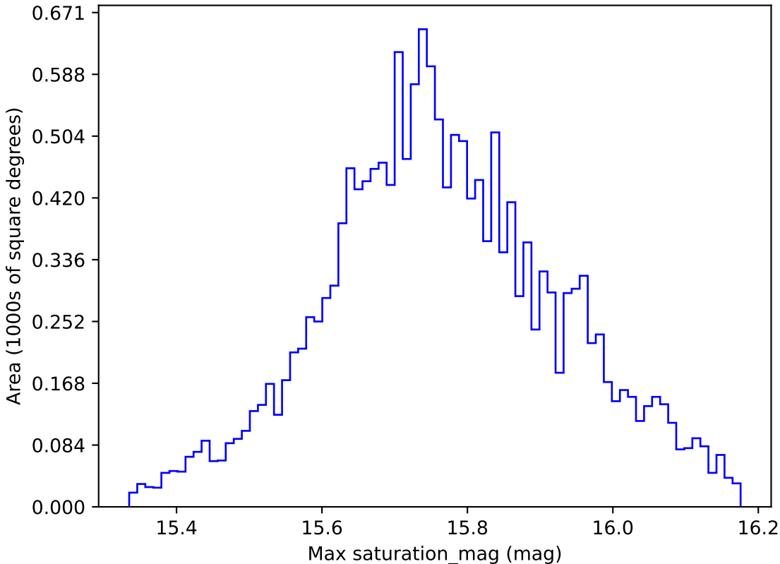
too_elab_r16_d3_giz_v3.4_10yrs WFD r band: Max saturation_mag
