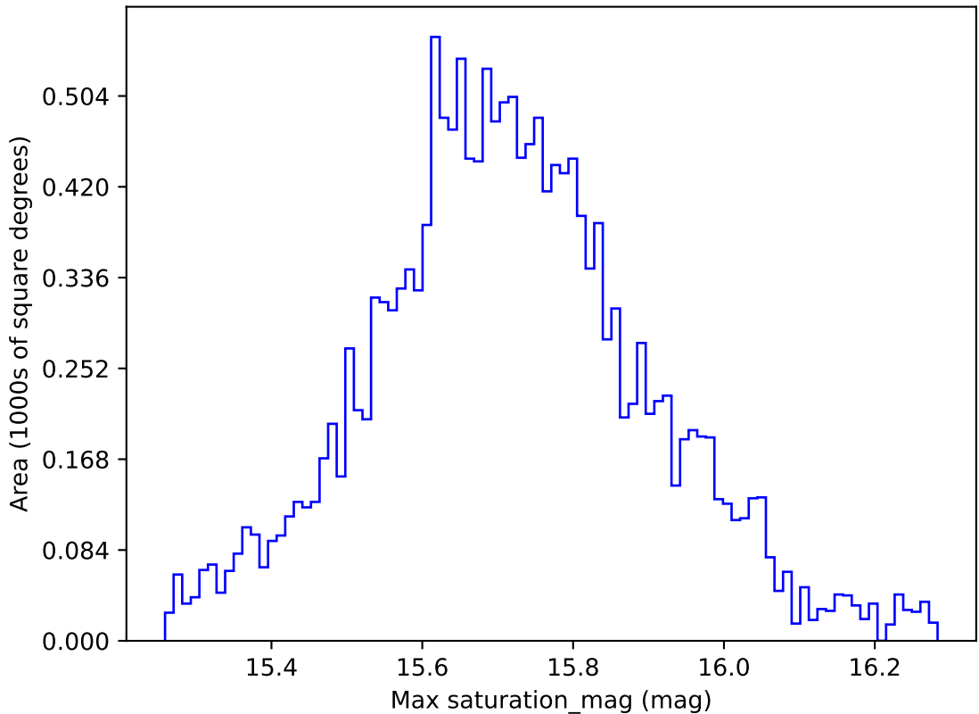
too_elab_r16_d3_giz_v3.4_10yrs WFD g band: Max saturation_mag
