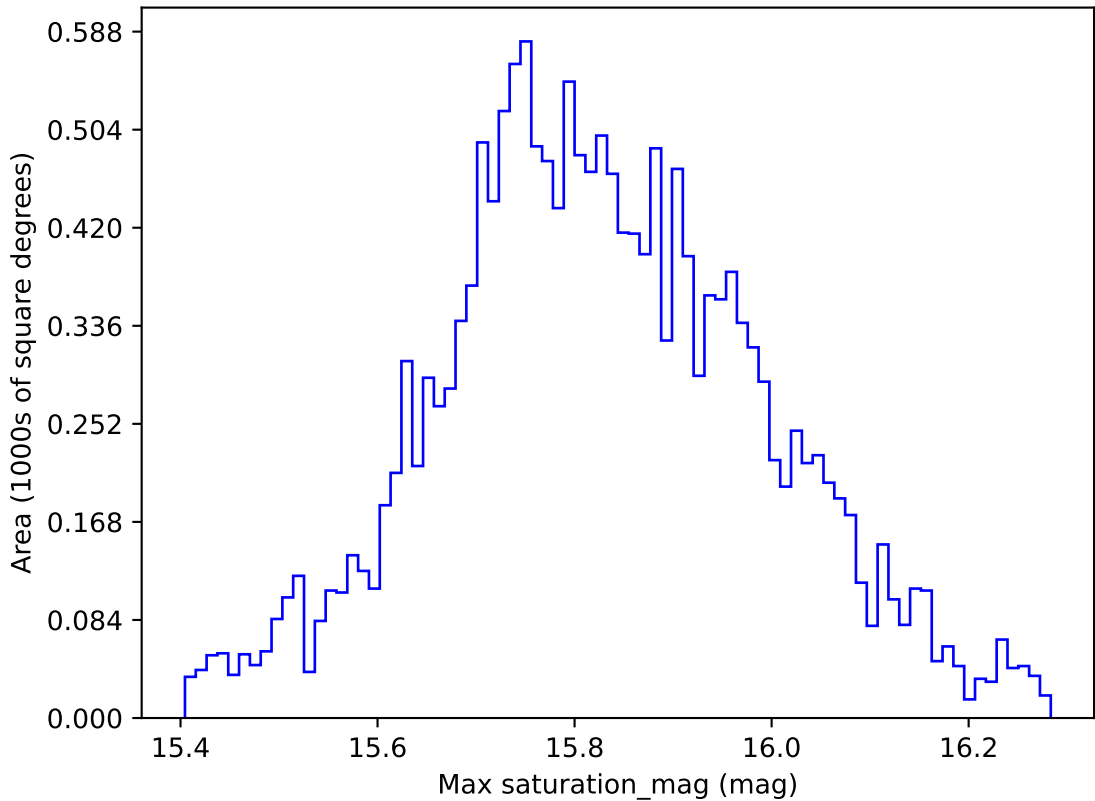
too_elab_r16_d3_giz_v3.4_10yrs WFD all bands: Max saturation_mag
