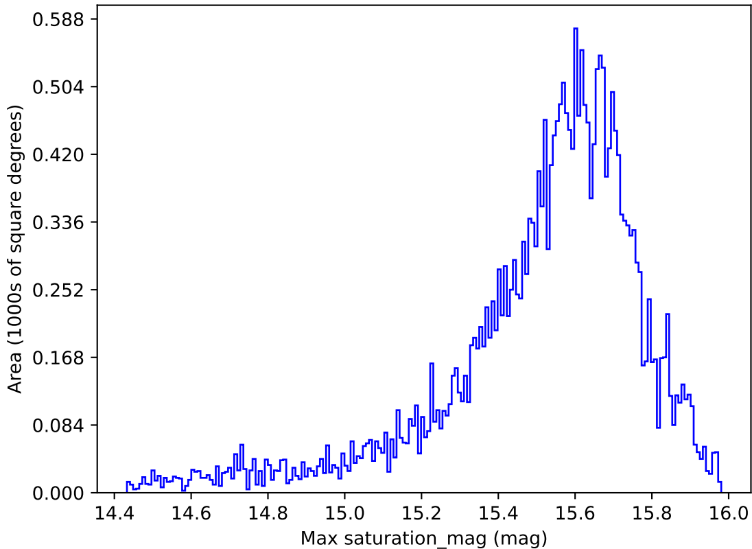
too_elab_r16_d3_giz_v3.4_10yrs All sky i band: Max saturation_mag
