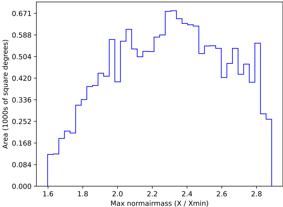
too_elab_r16_d3_giz_v3.4_10yrs WFD z band: Max normairmass
