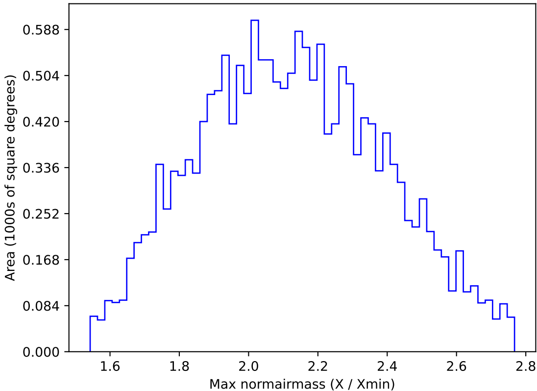
too_elab_r16_d3_giz_v3.4_10yrs WFD y band: Max normairmass
