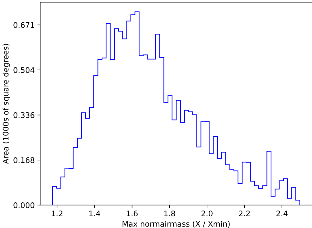
too_elab_r16_d3_giz_v3.4_10yrs WFD u band: Max normairmass
