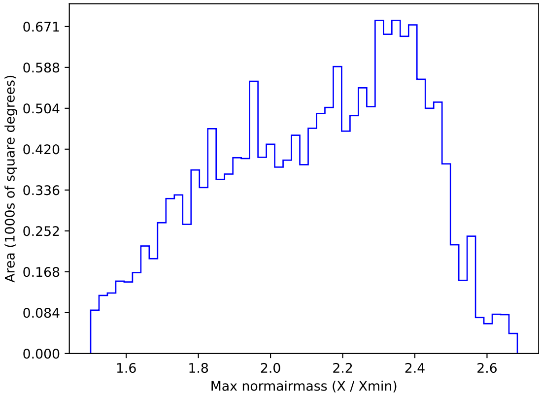
too_elab_r16_d3_giz_v3.4_10yrs WFD r band: Max normairmass
