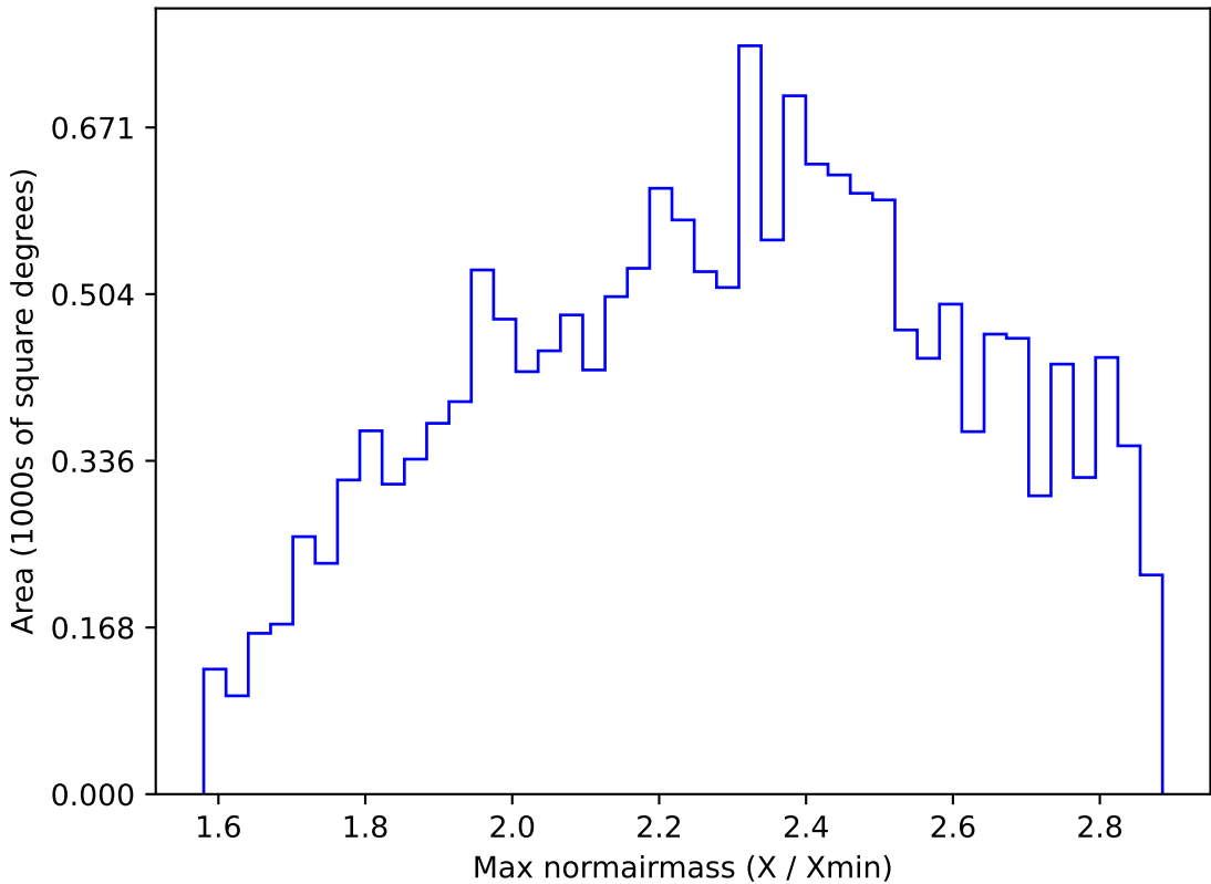
too_elab_r16_d3_giz_v3.4_10yrs WFD i band: Max normairmass
