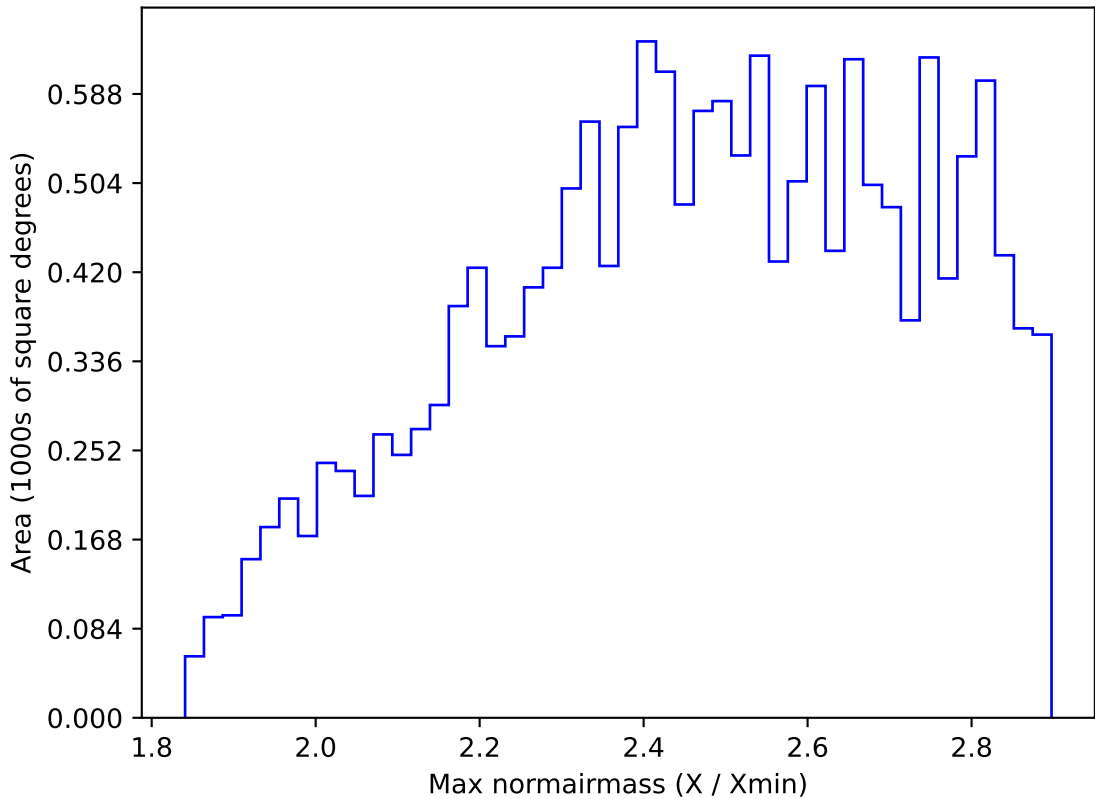
too_elab_r16_d3_giz_v3.4_10yrs WFD all bands: Max normairmass
