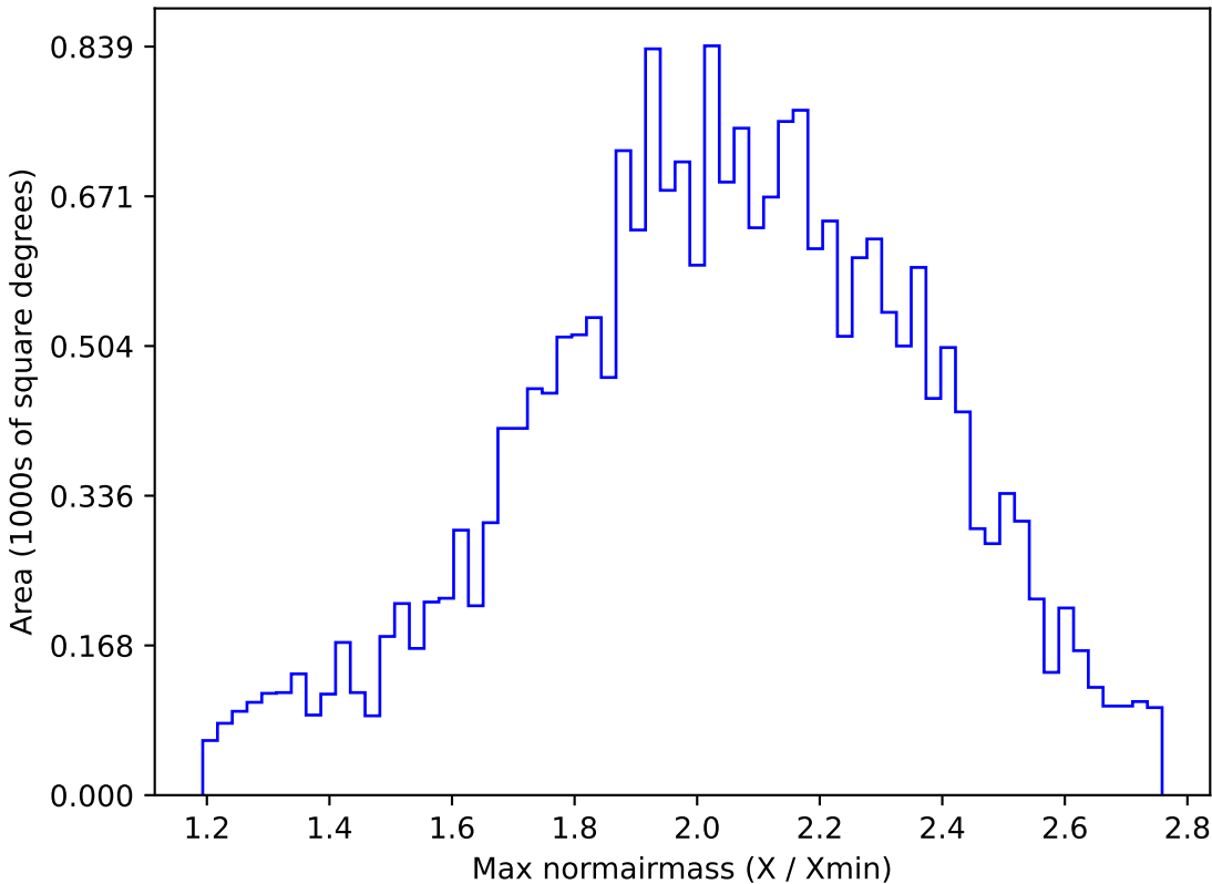
too_elab_r16_d3_giz_v3.4_10yrs All sky y band: Max normairmass
