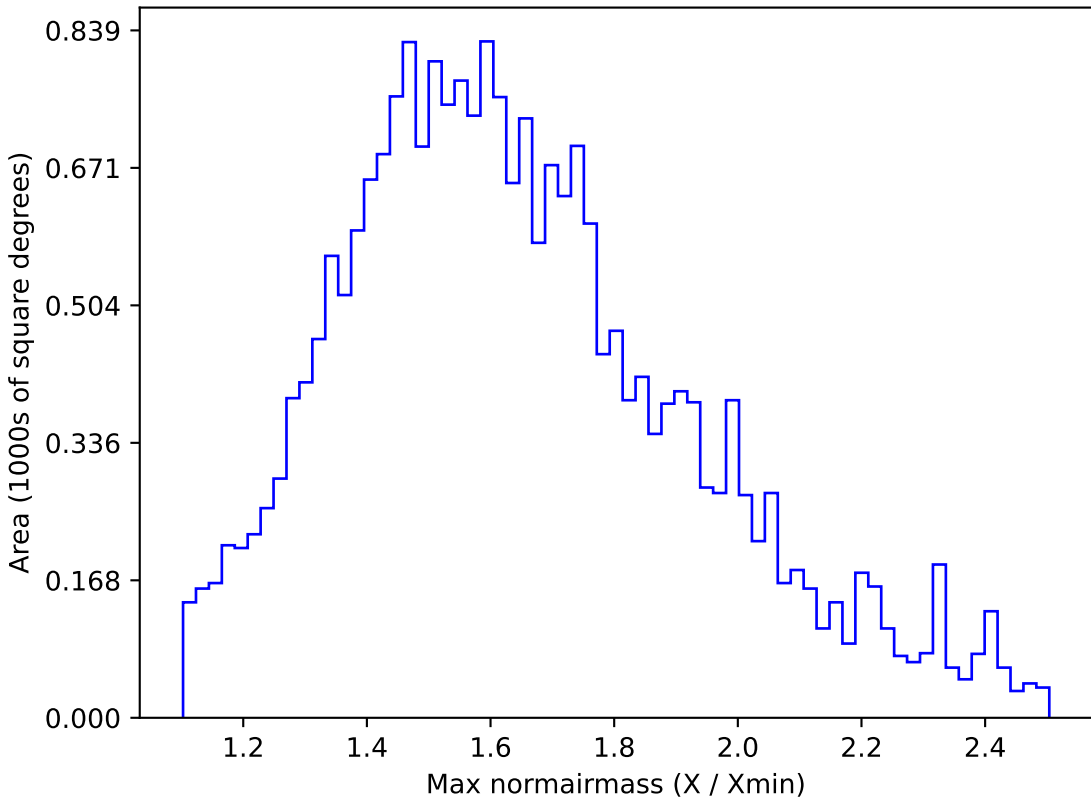
too_elab_r16_d3_giz_v3.4_10yrs All sky u band: Max normairmass
