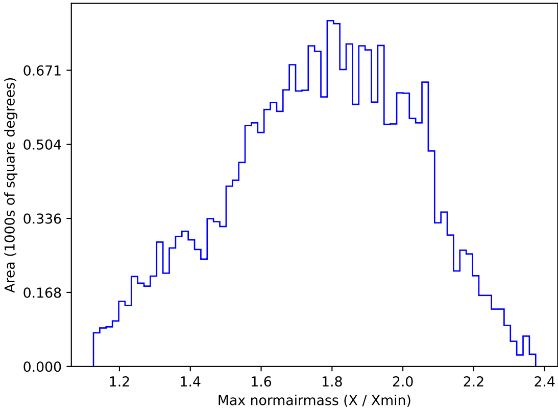
too_elab_r16_d3_giz_v3.4_10yrs All sky g band: Max normairmass
