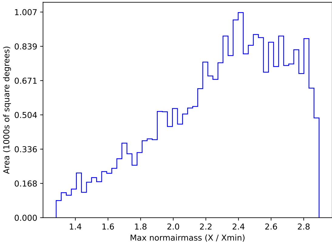
too_elab_r16_d3_giz_v3.4_10yrs All sky all bands: Max normairmass
