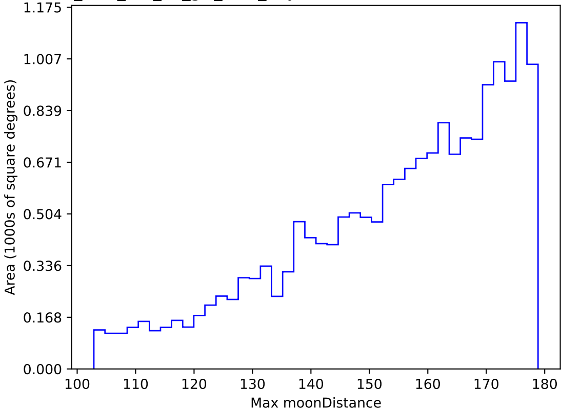
too_elab_r16_d3_giz_v3.4_10yrs WFD z band: Max moonDistance
