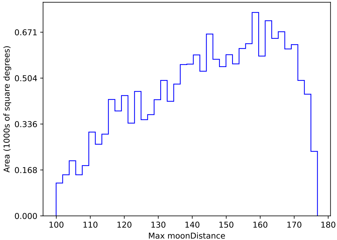
too_elab_r16_d3_giz_v3.4_10yrs WFD y band: Max moonDistance
