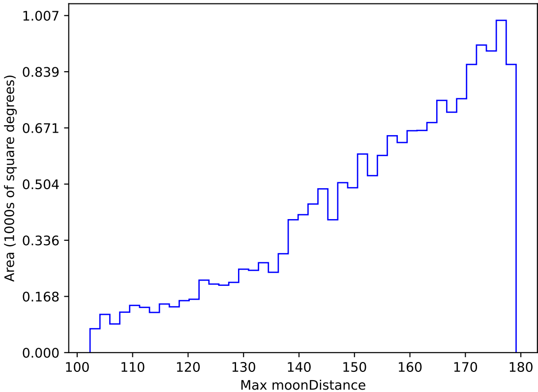
too_elab_r16_d3_giz_v3.4_10yrs WFD u band: Max moonDistance
