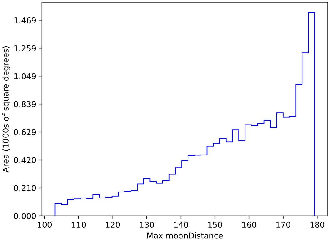
too_elab_r16_d3_giz_v3.4_10yrs WFD r band: Max moonDistance
