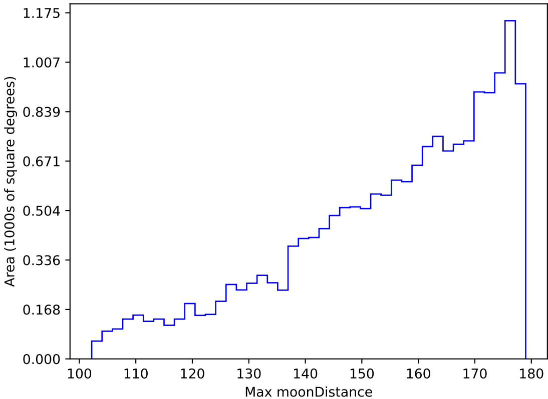
too_elab_r16_d3_giz_v3.4_10yrs WFD g band: Max moonDistance
