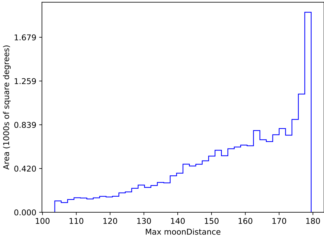
too_elab_r16_d3_giz_v3.4_10yrs WFD all bands: Max moonDistance
