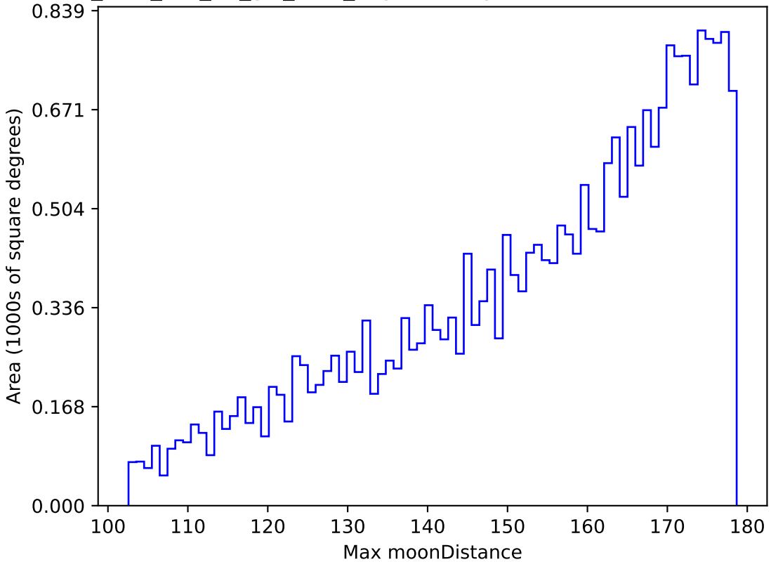
too_elab_r16_d3_giz_v3.4_10yrs All sky z band: Max moonDistance
