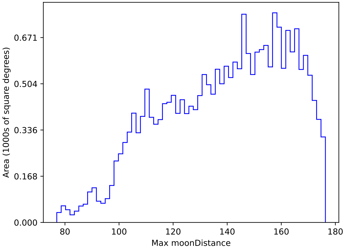
too_elab_r16_d3_giz_v3.4_10yrs All sky y band: Max moonDistance
