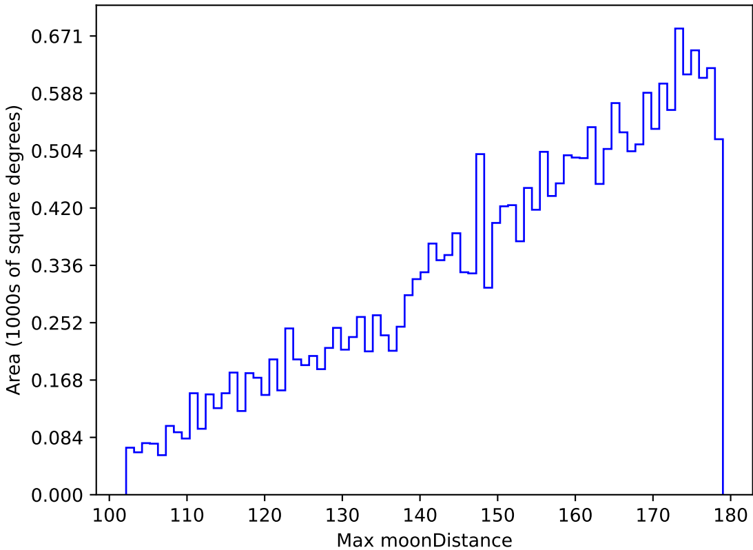
too_elab_r16_d3_giz_v3.4_10yrs All sky u band: Max moonDistance
