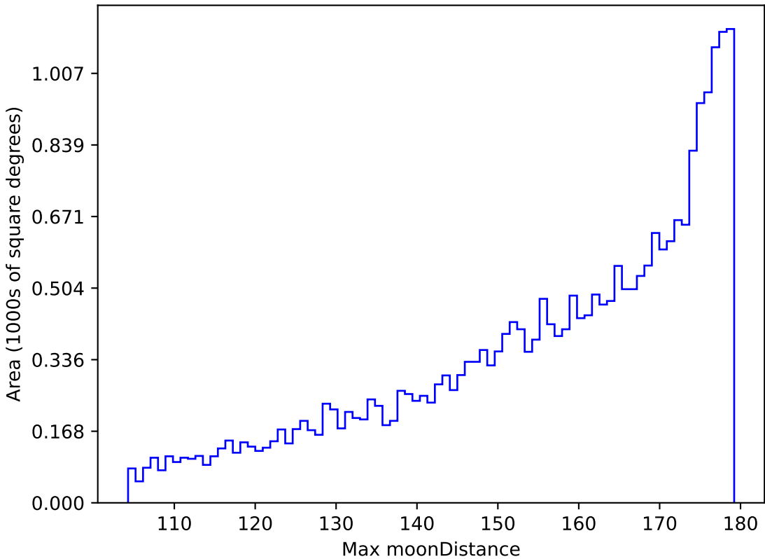
too_elab_r16_d3_giz_v3.4_10yrs All sky r band: Max moonDistance
