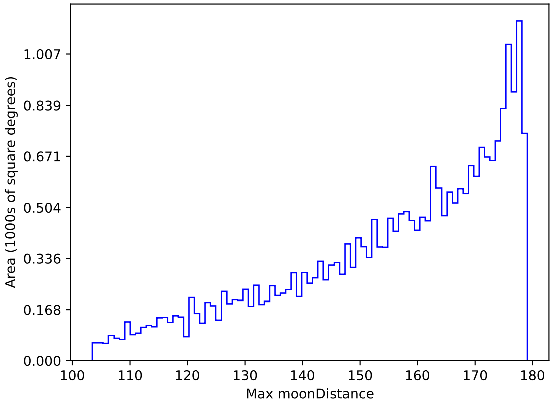
too_elab_r16_d3_giz_v3.4_10yrs All sky i band: Max moonDistance
