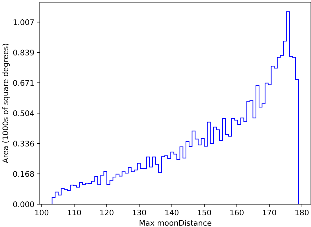
too_elab_r16_d3_giz_v3.4_10yrs All sky g band: Max moonDistance
