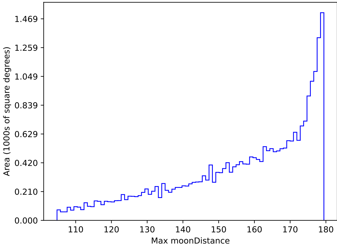
too_elab_r16_d3_giz_v3.4_10yrs All sky all bands: Max moonDistance
