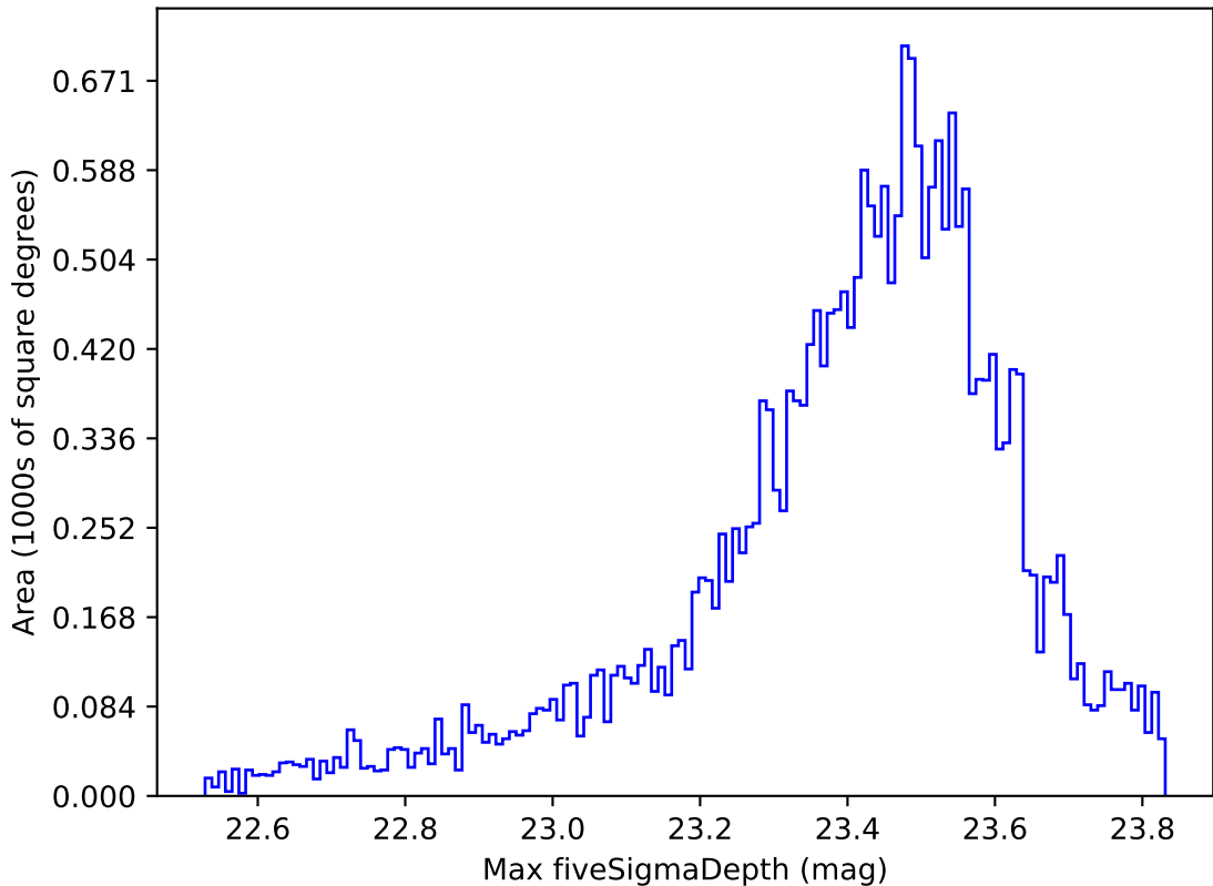
too_elab_r16_d3_giz_v3.4_10yrs Yr 1 z band: Max fiveSigmaDepth
