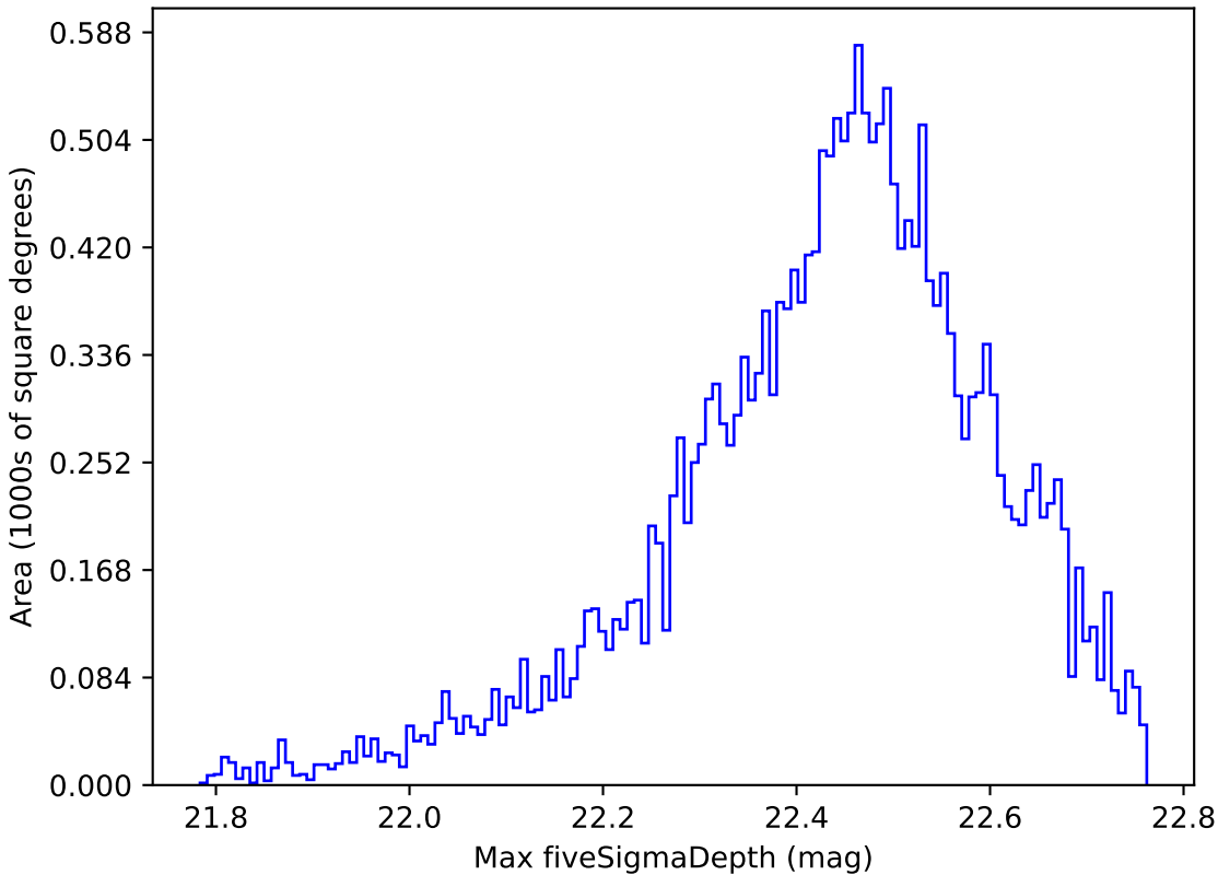
too_elab_r16_d3_giz_v3.4_10yrs Yr 1 y band: Max fiveSigmaDepth
