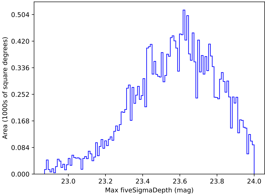
too_elab_r16_d3_giz_v3.4_10yrs Yr 1 u band: Max fiveSigmaDepth
