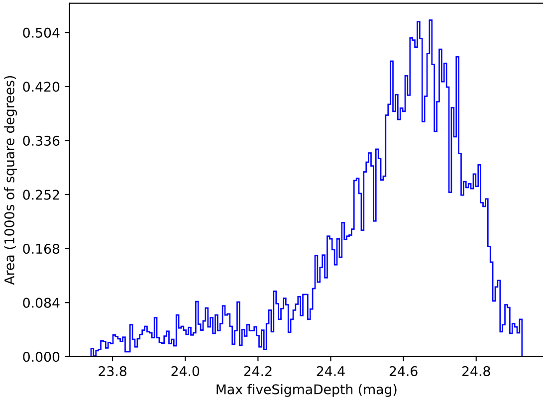
too_elab_r16_d3_giz_v3.4_10yrs Yr 1 r band: Max fiveSigmaDepth
