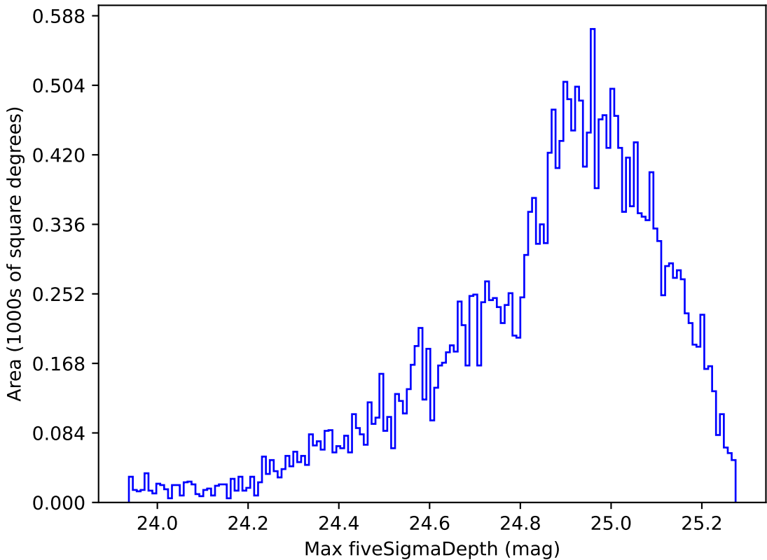
too_elab_r16_d3_giz_v3.4_10yrs Yr 1 g band: Max fiveSigmaDepth
