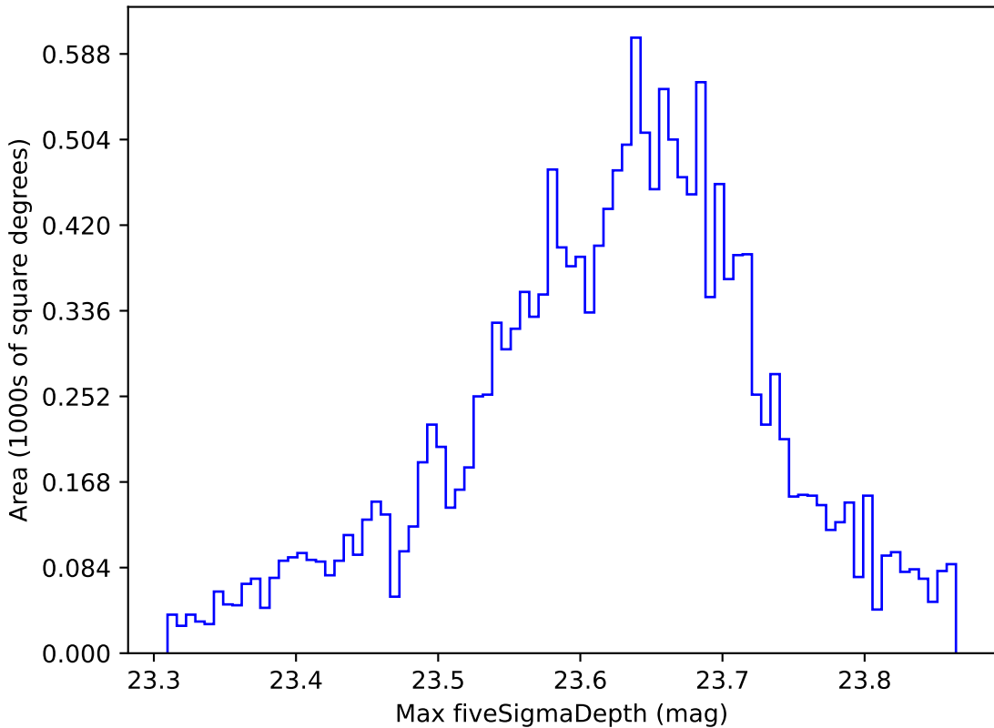
too_elab_r16_d3_giz_v3.4_10yrs WFD z band: Max fiveSigmaDepth
