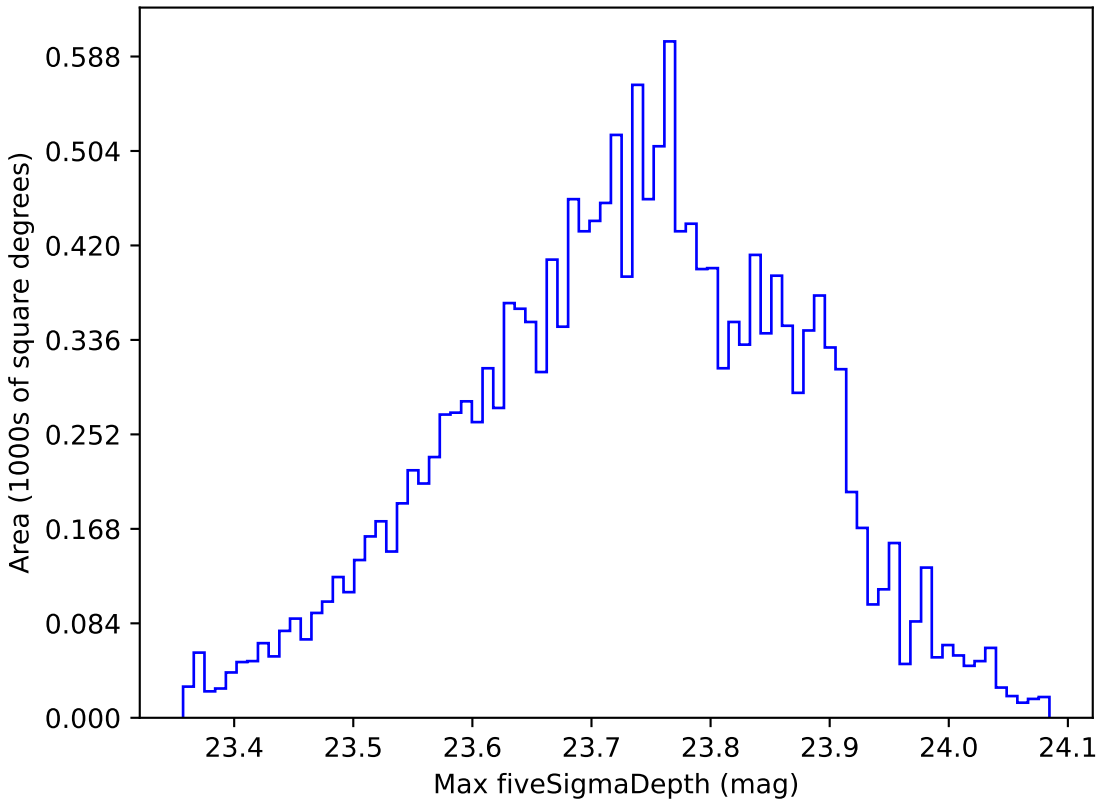
too_elab_r16_d3_giz_v3.4_10yrs WFD u band: Max fiveSigmaDepth
