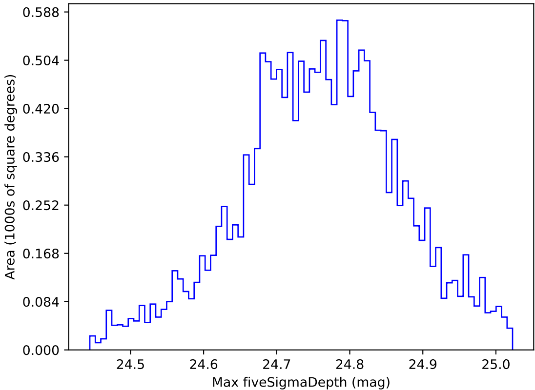
too_elab_r16_d3_giz_v3.4_10yrs WFD r band: Max fiveSigmaDepth
