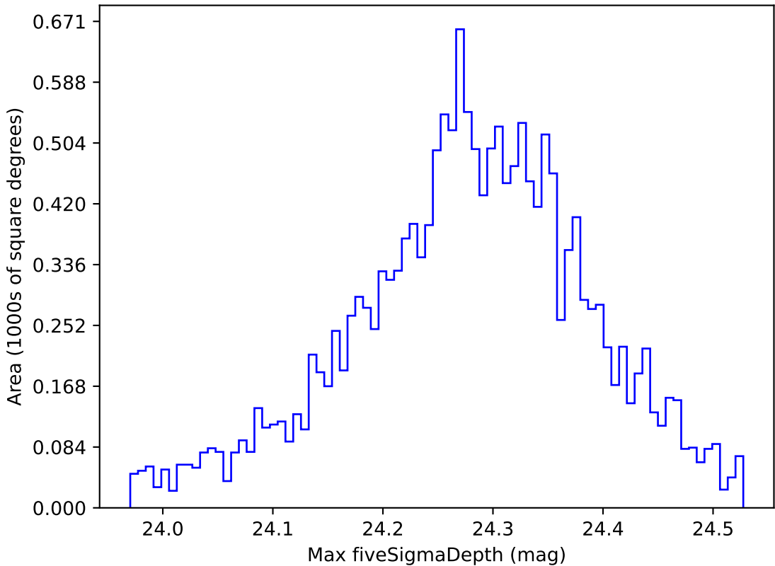
too_elab_r16_d3_giz_v3.4_10yrs WFD i band: Max fiveSigmaDepth
