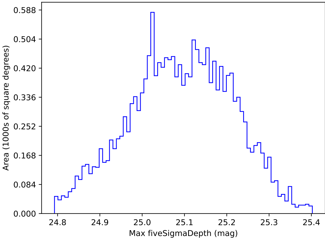
too_elab_r16_d3_giz_v3.4_10yrs WFD g band: Max fiveSigmaDepth
