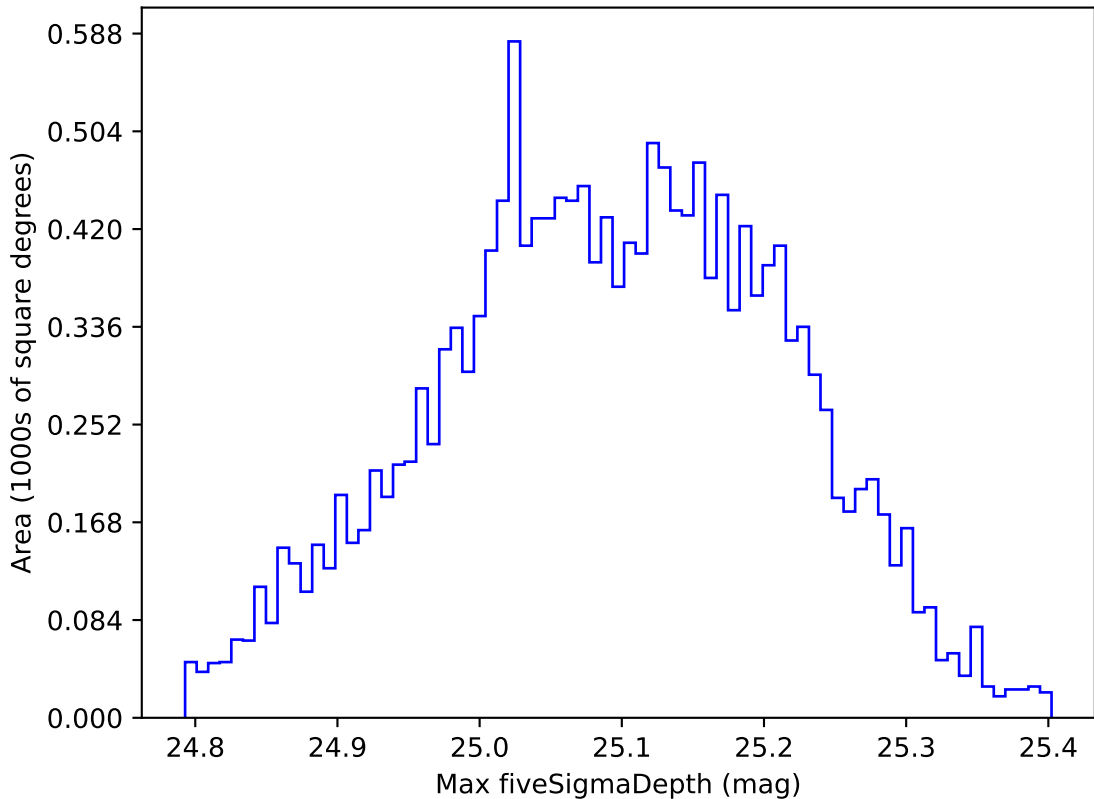
too_elab_r16_d3_giz_v3.4_10yrs WFD all bands: Max fiveSigmaDepth
