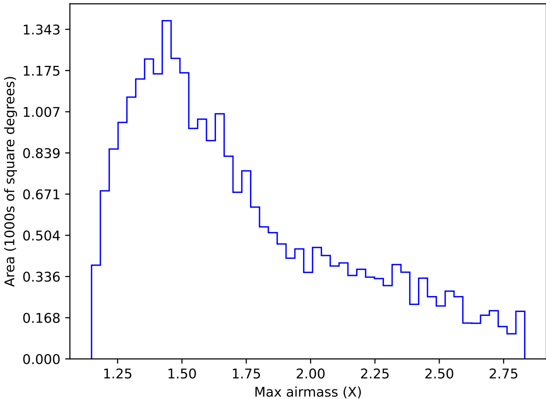
too_elab_r16_d3_giz_v3.4_10yrs Yr 1 z band: Max airmass
