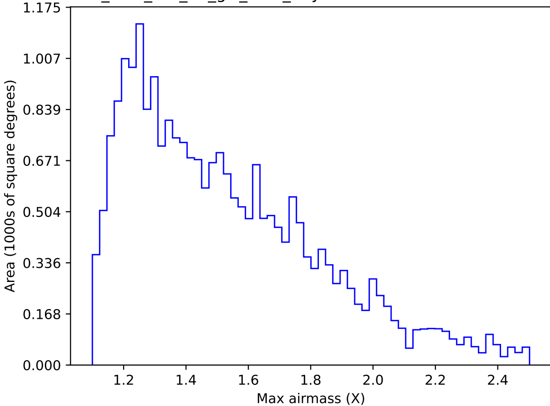
too_elab_r16_d3_giz_v3.4_10yrs Yr 1 u band: Max airmass
