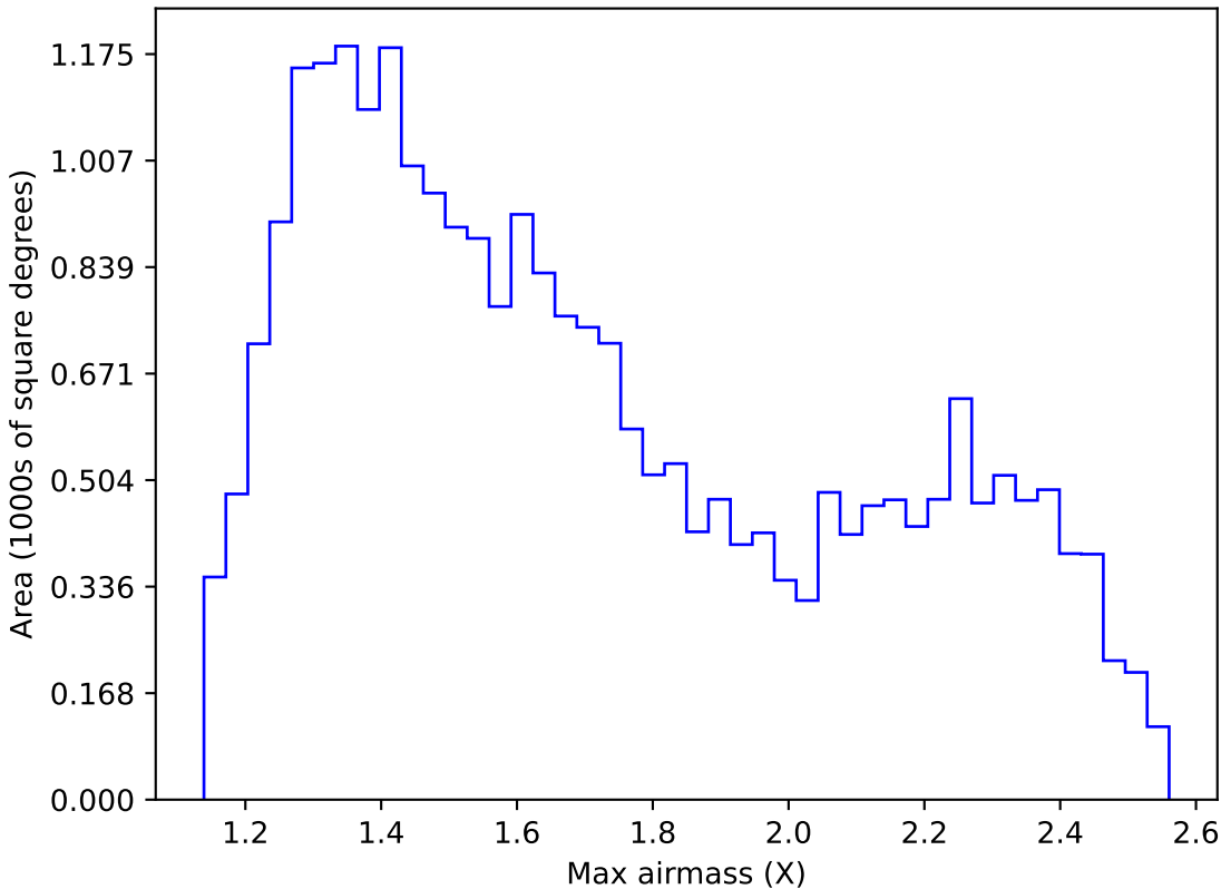
too_elab_r16_d3_giz_v3.4_10yrs Yr 1 r band: Max airmass
