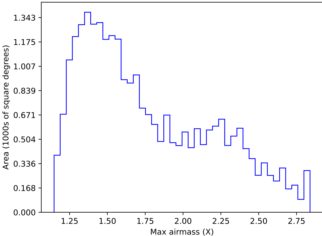
too_elab_r16_d3_giz_v3.4_10yrs Yr 1 i band: Max airmass
