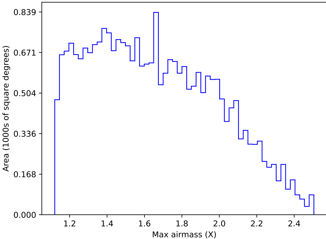
too_elab_r16_d3_giz_v3.4_10yrs Yr 1 g band: Max airmass
