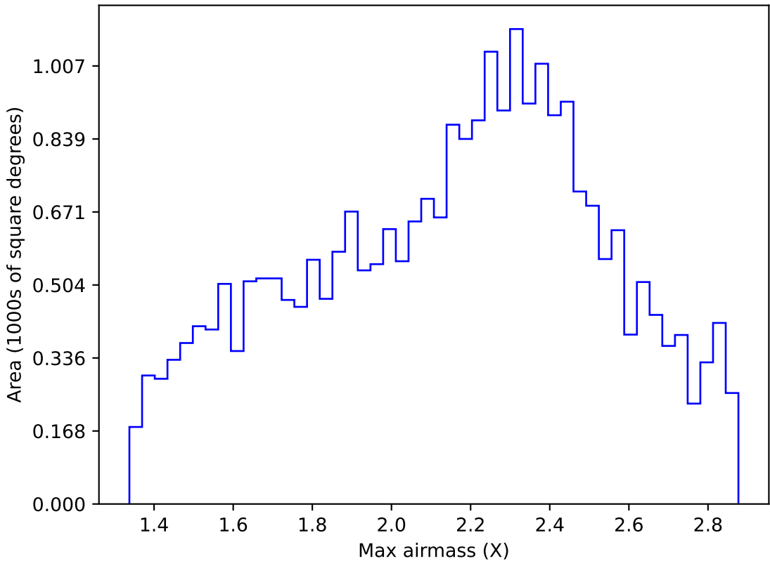
too_elab_r16_d3_giz_v3.4_10yrs Yr 1 all bands: Max airmass
