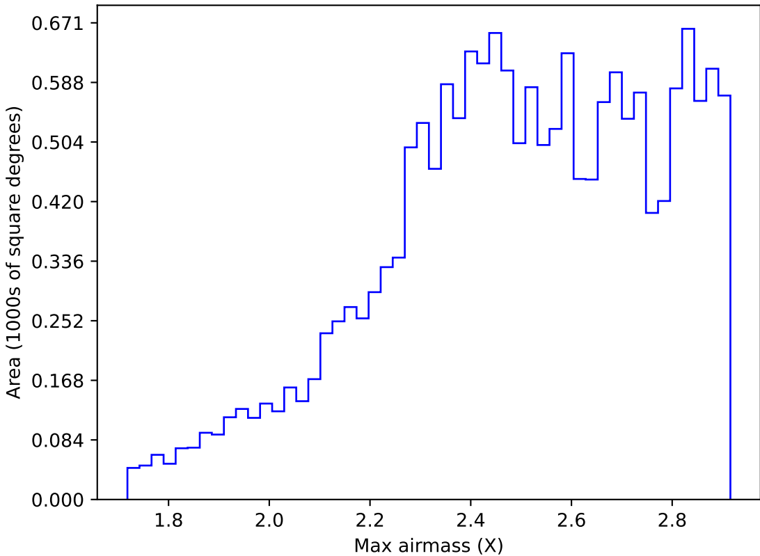
too_elab_r16_d3_giz_v3.4_10yrs WFD z band: Max airmass
