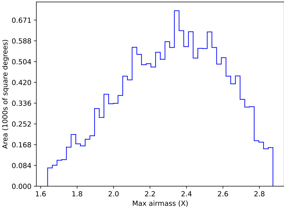
too_elab_r16_d3_giz_v3.4_10yrs WFD y band: Max airmass
