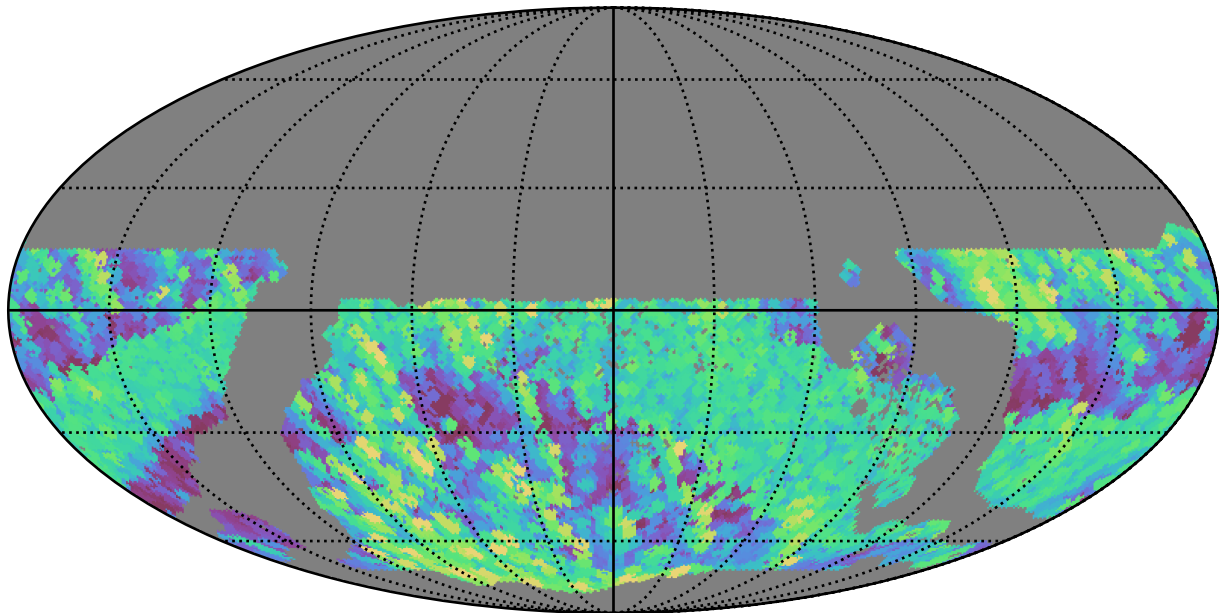
too_elab_r16_d3_giz_v3.4_10yrs WFD r band: Max airmass
